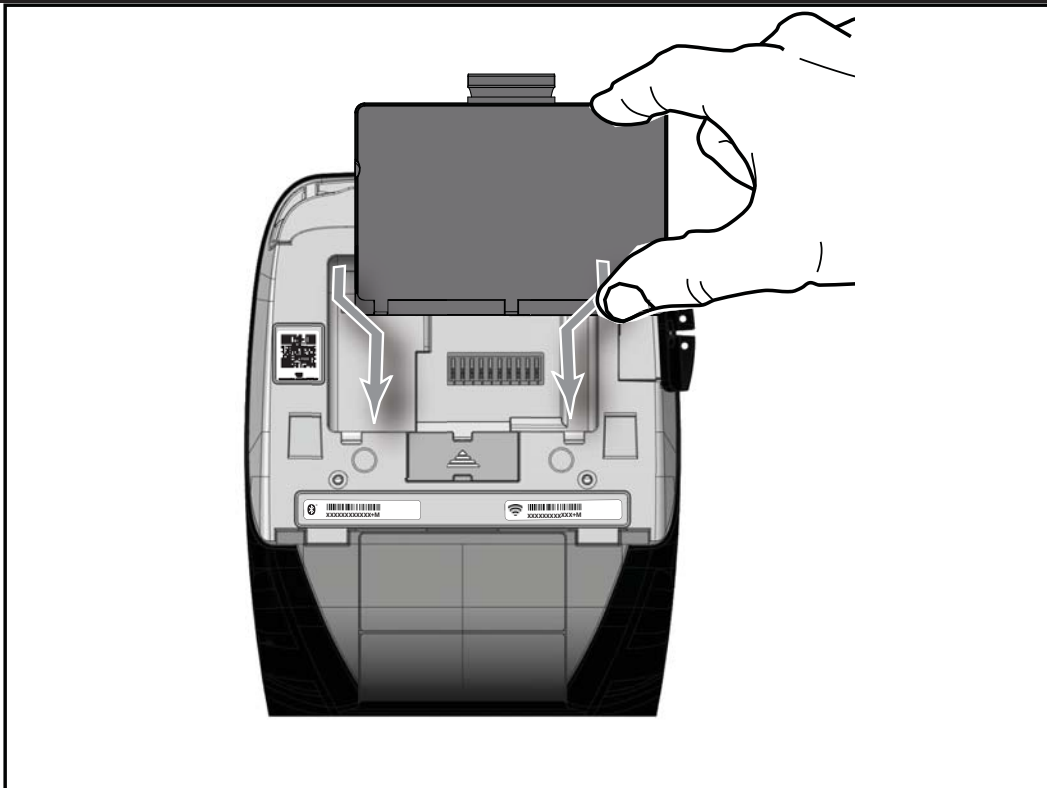
Figure 1: Installing the Battery (ZQ510 Shown)
