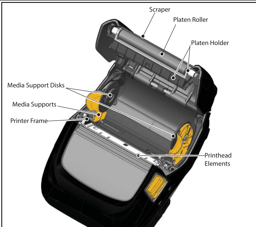
Figure 20b: Cleaning the ZQ500 Series Printers (Linerless)
