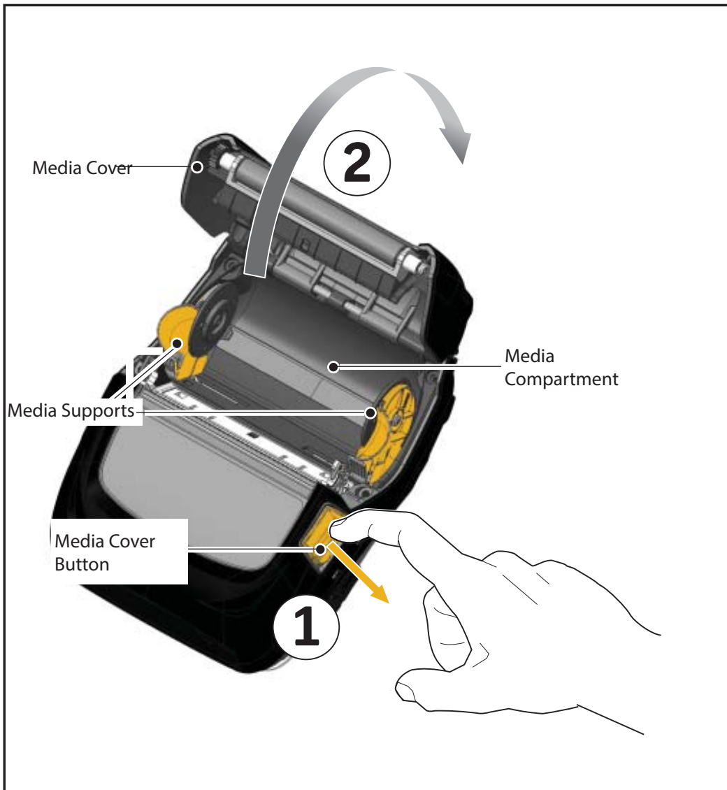
Figure 7: Opening the Printer
