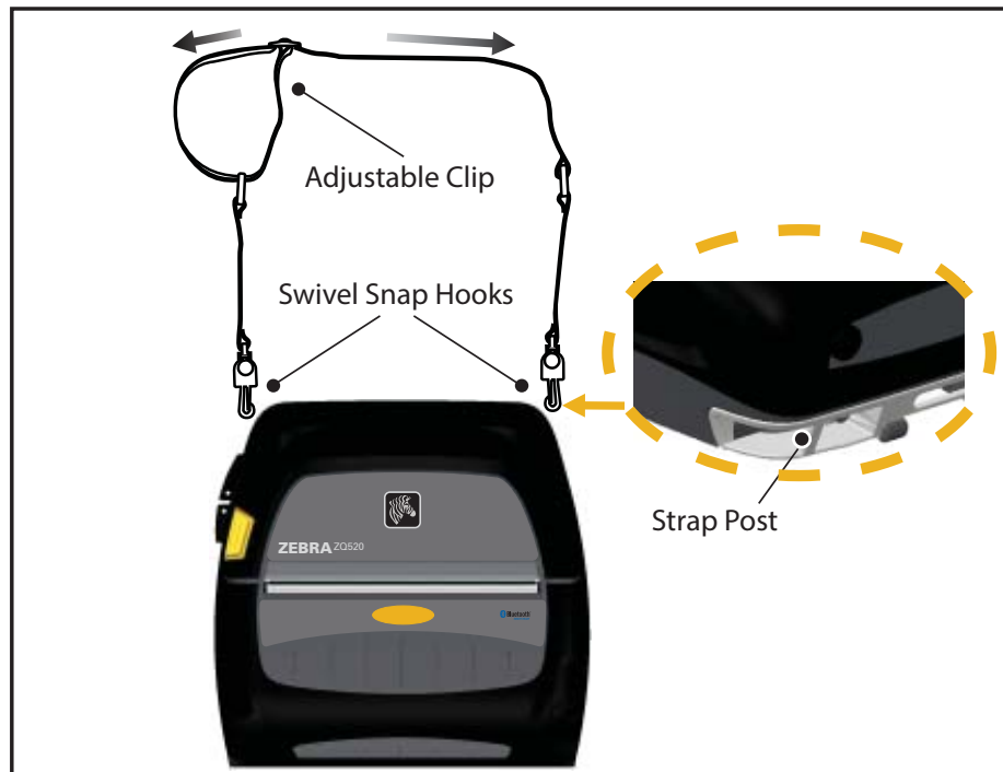
Figure 17: Using the Shoulder Strap
