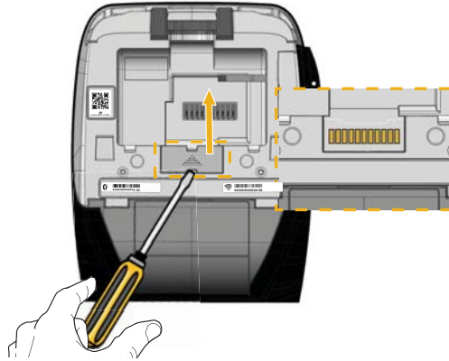
Figure 5: Docking and Un-Docking the Vehicle Cradle
