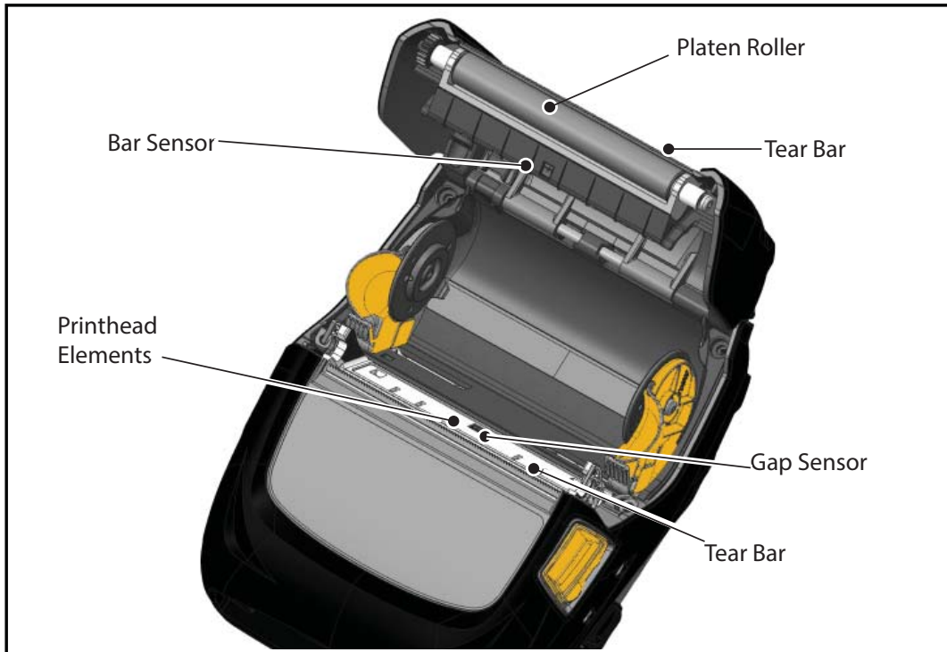
Figure 20a: Cleaning the ZQ500 Series Printers (Linered)
