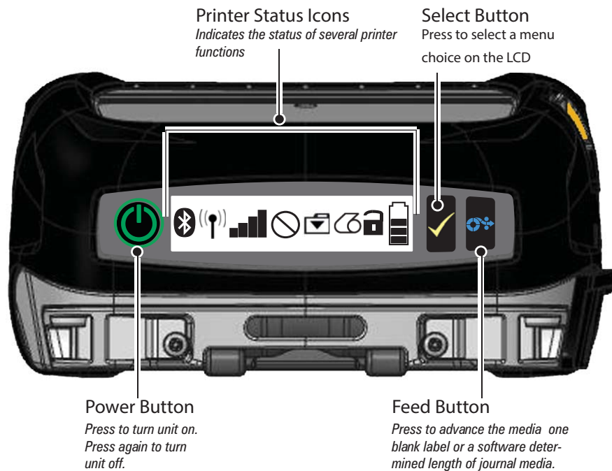
Figure 9: Control Panel
