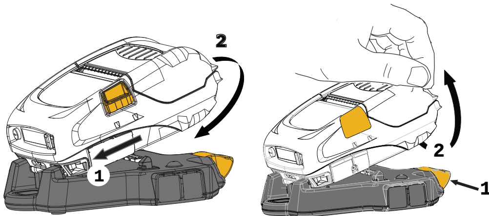
Figure 5: Docking and Un-Docking the Vehicle Cradle
