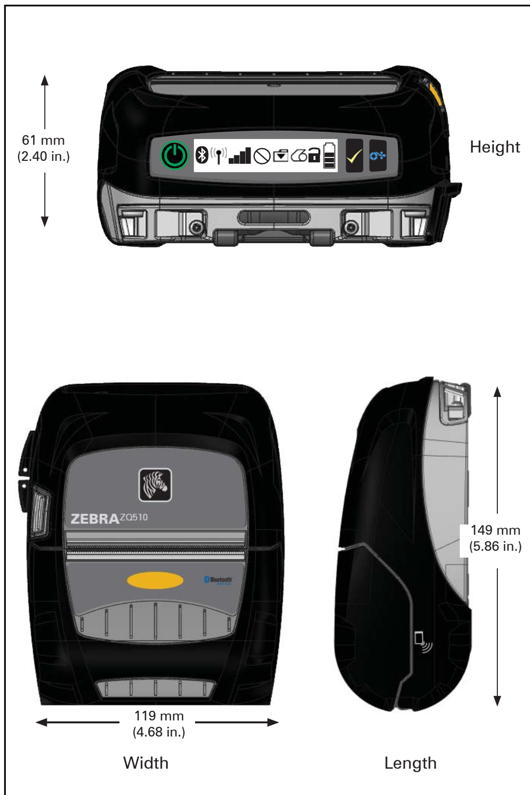
Figure 22: ZQ510 Overall Dimensions
