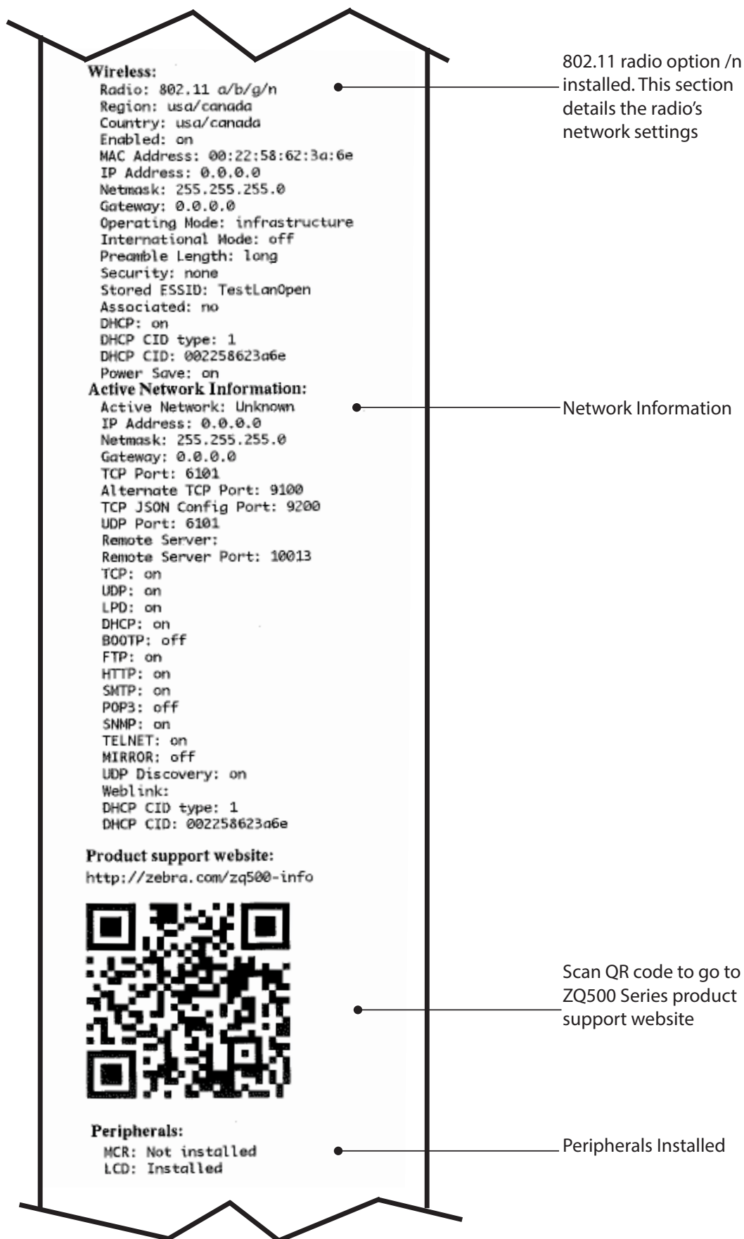
Figure 21b: ZQ500 Series Configuration Label (cont.)
