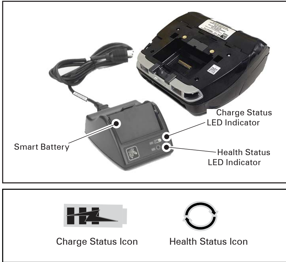
Figure 2: Smart Charger-2 (SC2)
