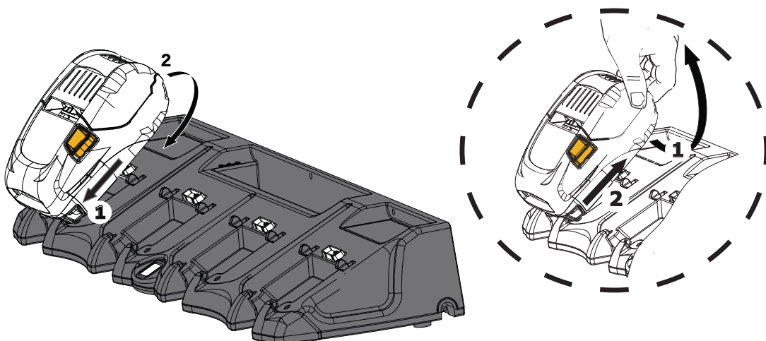
Figure 6: Docking and Un-Docking the 4-Bay Power Station
