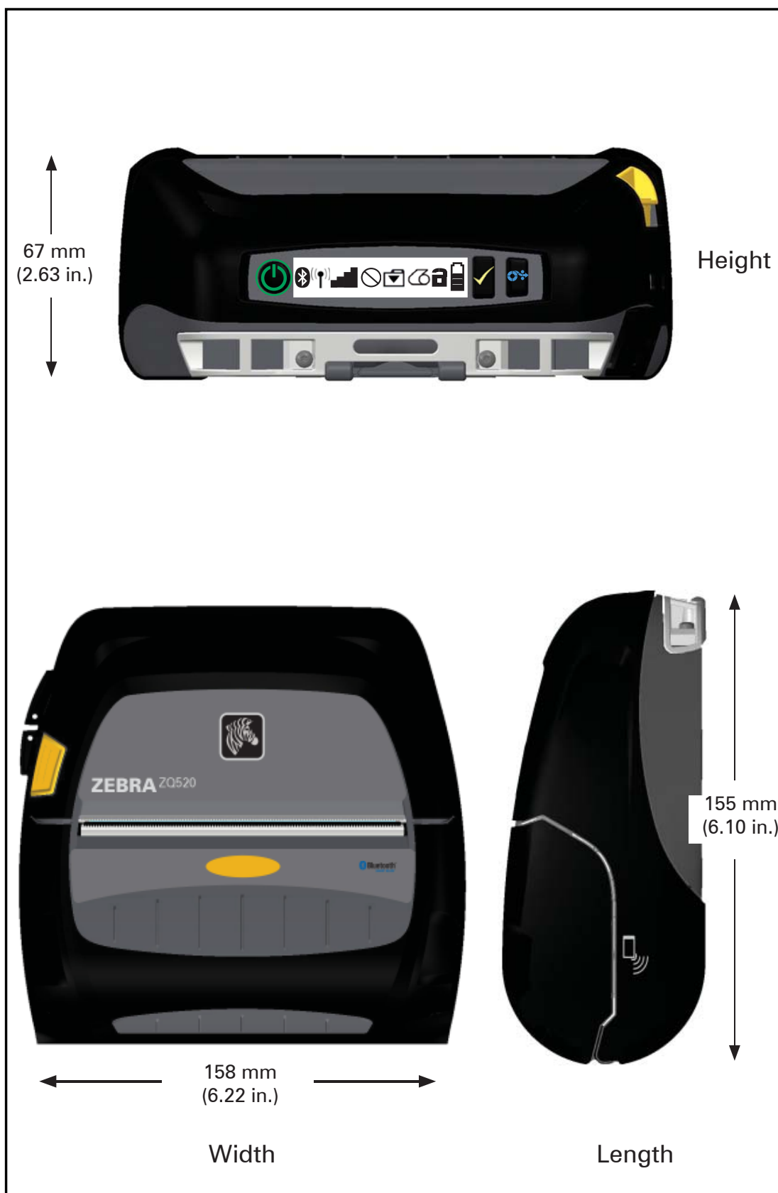
Figure 23: ZQ520 Overall Dimensions
