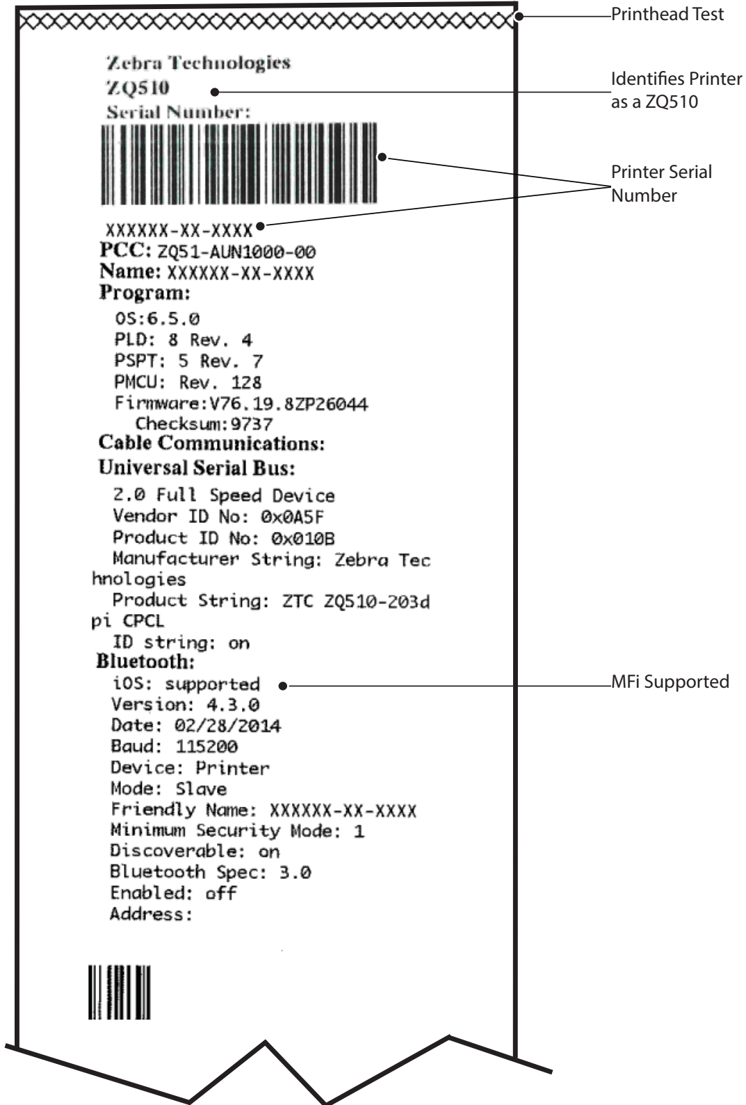
Figure 21a: ZQ500 Series Configuration Label (ZQ510 Shown)
