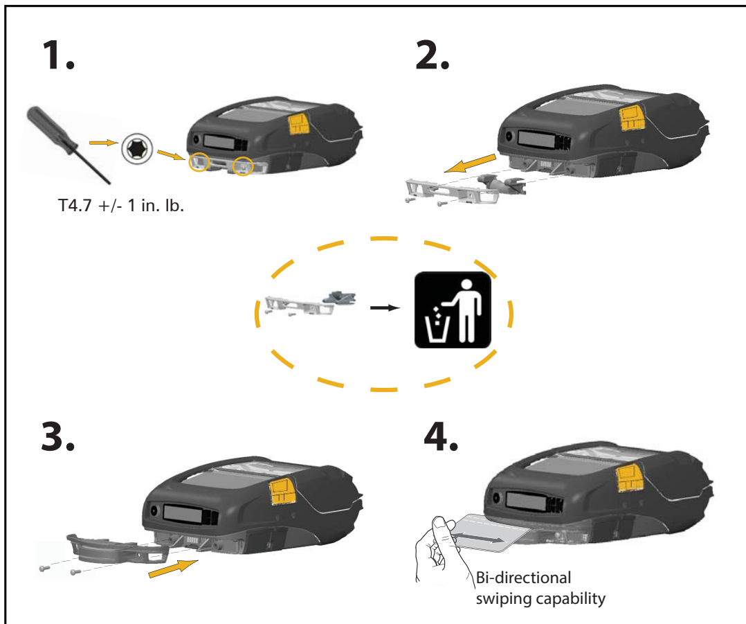
Figure 19: Installing the Mag Card Reader
