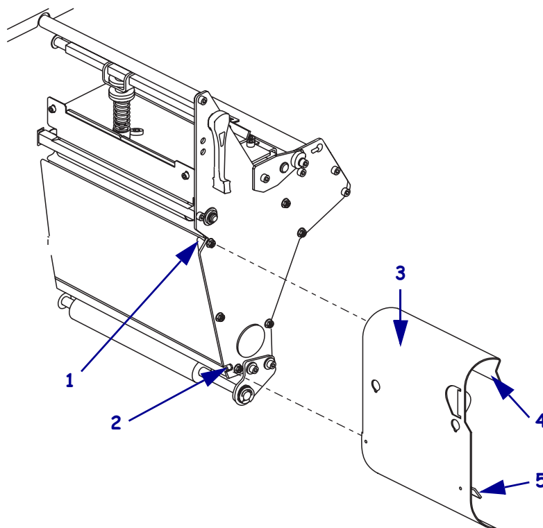
Figure 23 • Rewind Plate
