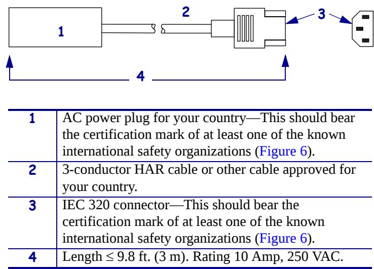
Figure 5 • Power Cord Specifications
