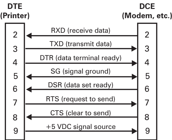
Figure 40 • RS-232 Cable Connections
