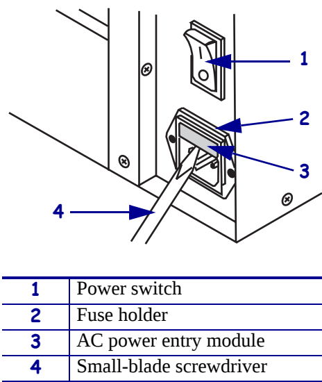
Figure 29 • AC Power Entry Module
