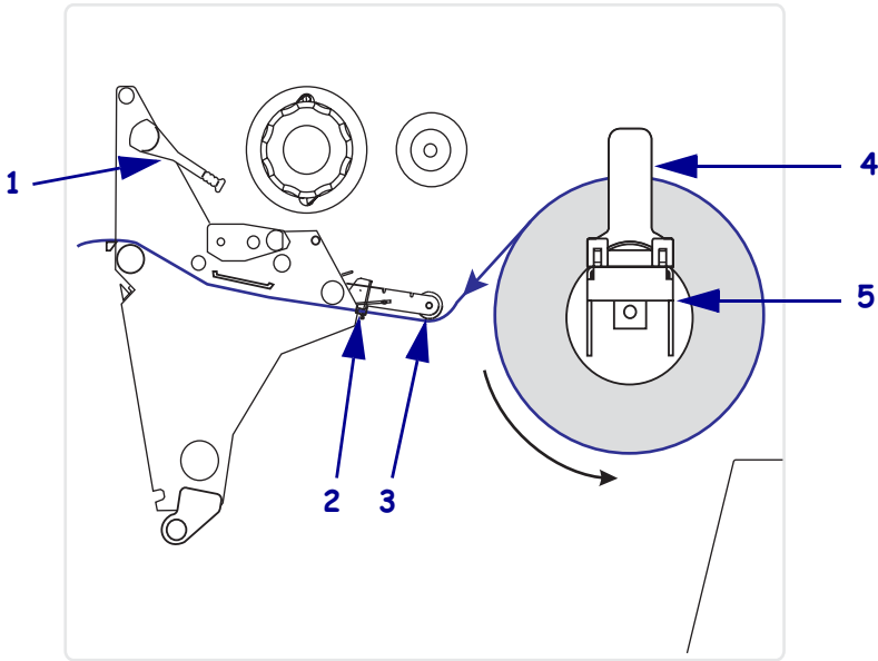
Figure 10 • Tear-Off Mode
