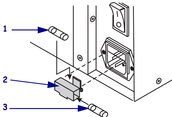
Figure 30 • Fuse Locations
