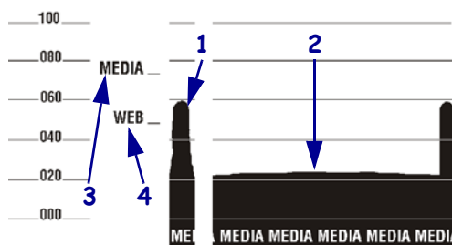
Figure 37 • Sensor Profile (Media Section)
