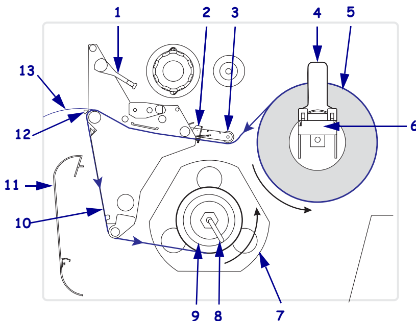
Figure 19 • Media Loaded in Peel-Off Mode
