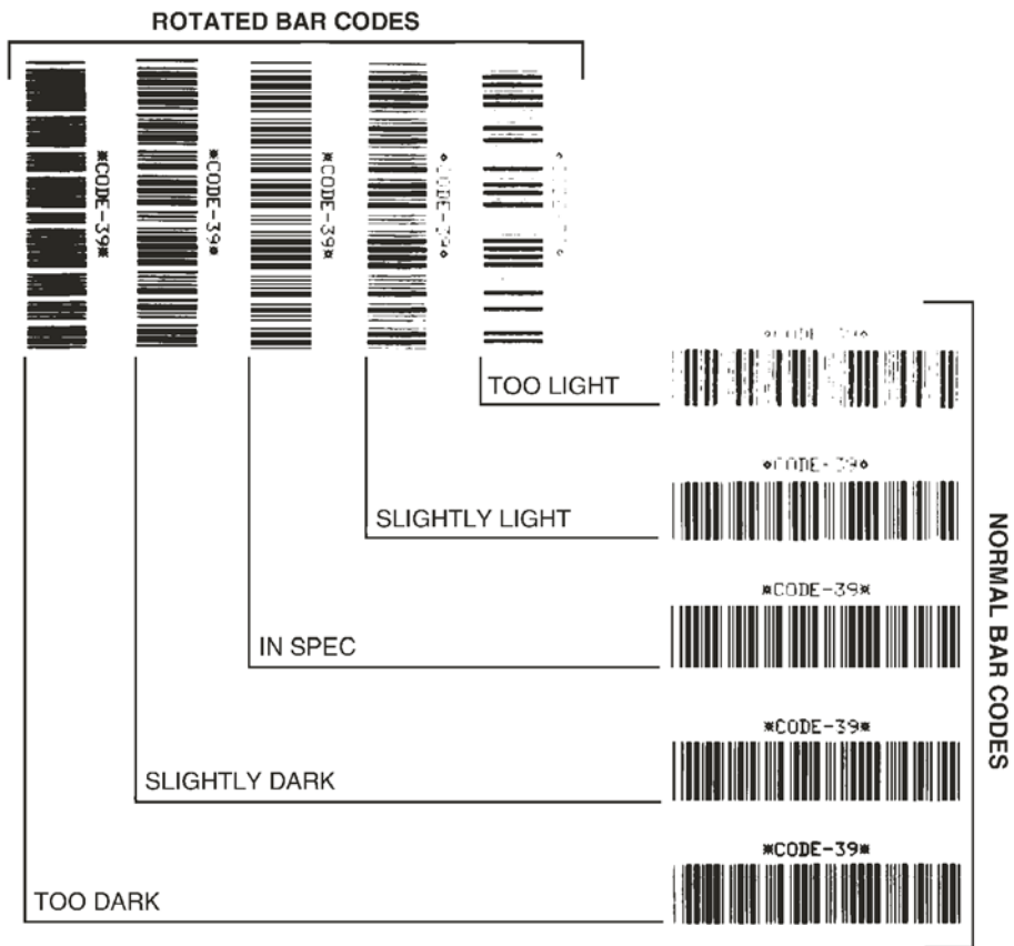
Figure 34 • Bar Code Darkness Comparison
